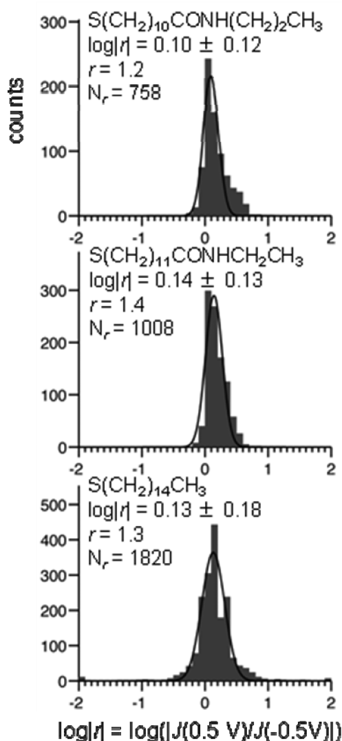
Figure 4. Histograms of \log|r| , where r = J(0.5 \text{ V})/J(-0.5 \text{ V}) , for compounds with amides at near the terminal group closer to the top electrode and for n -alkanethiols. All compounds have 15 non-H atoms in the molecular backbone (excluding sulfur). The first two histograms illustrate the effect of having an amide, and/or shifting the amide by a single carbon, while the bottom histogram is from an n -alkanethiol of similar length (same barrier width) for reference.
