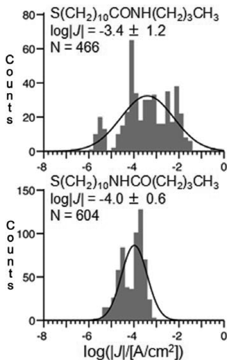
Figure 3. Histograms of \log |J| for two alkyl amides, 10,4 and 10,4* , compounds in which the orientation of the amide has been reversed but the total length of the molecule is the same. The spreads in the distributions for the two compounds overlap, making the averages of \log |J| indistinguishable.
