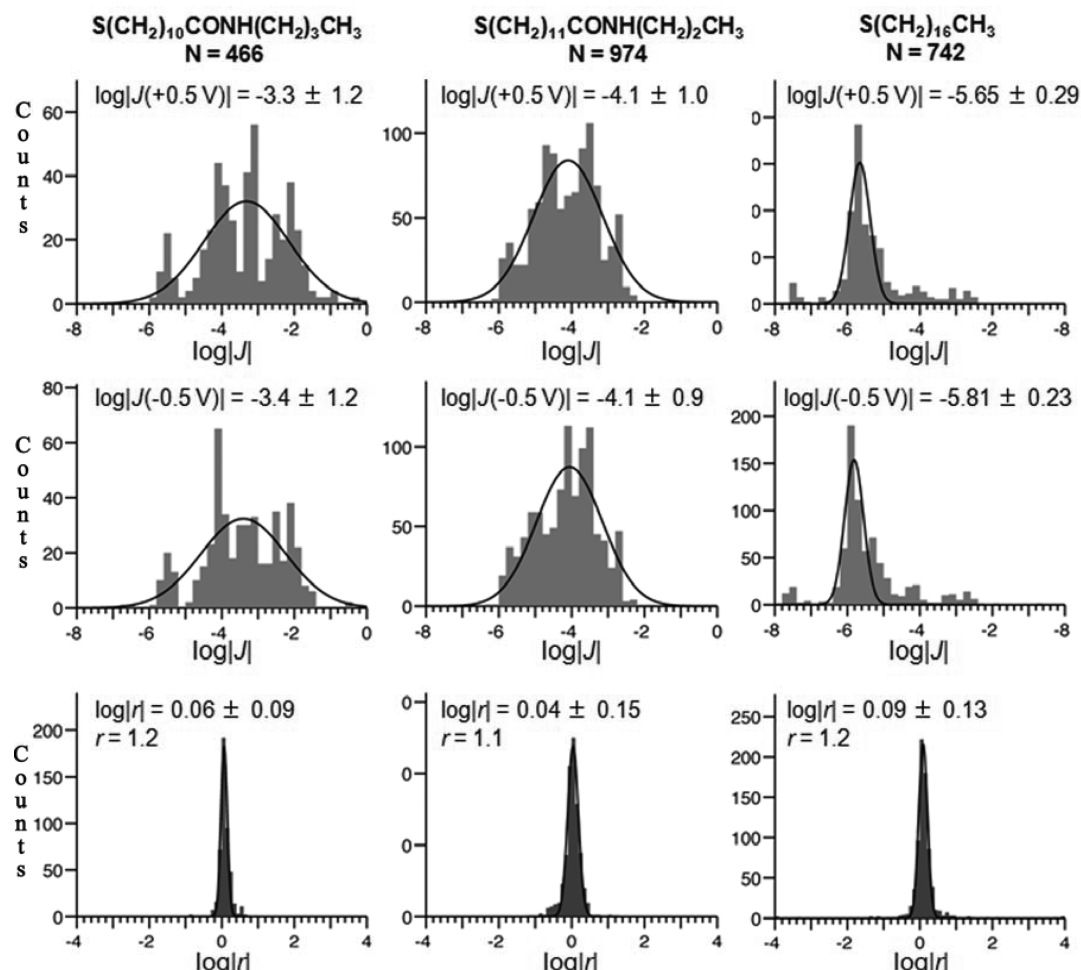
Figure 5. Histograms of \log|J| at opposite biases, +0.5 V (top row) and -0.5 V (middle row), above those of \log|r| (bottom row), where r = J(+0.5\text{ V})/J(-0.5\text{ V}) , for two compounds with internal amides along the molecular backbone and an n -alkanethiol. The first two rows of histograms illustrate the effect of reversing the applied bias on the distribution of the histograms. The bottom row of histograms gives the histogram of rectification ratios for the three molecules. Comparison down each column illustrates the difference between the width of distributions for current density at opposite applied biases and the rectification ratios.
